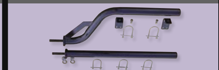
M-RTF-60 Universal offset style bolt-on fender mount kit
