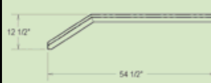
STF-60 Standard Half Fender Use M-RTF-60 mounting kit
