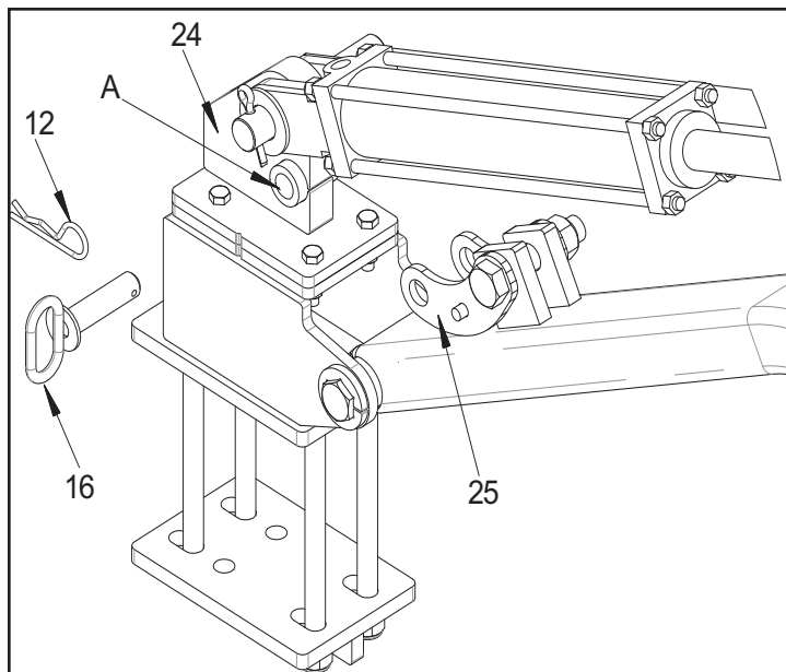
Figure 3.4 - Transport Lock
